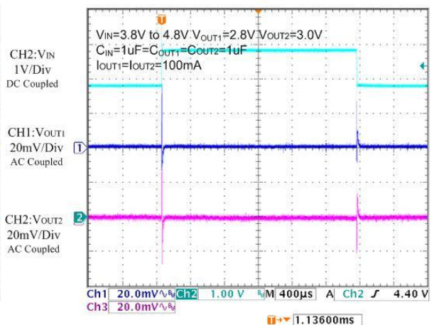
Line Transient
